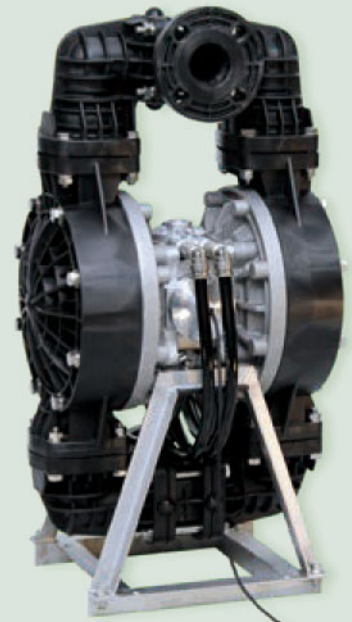
D400V□J-EX 1 1/2" CFPVDF E Type Pump (Flanged) 350 L/min Max Flow Rate
